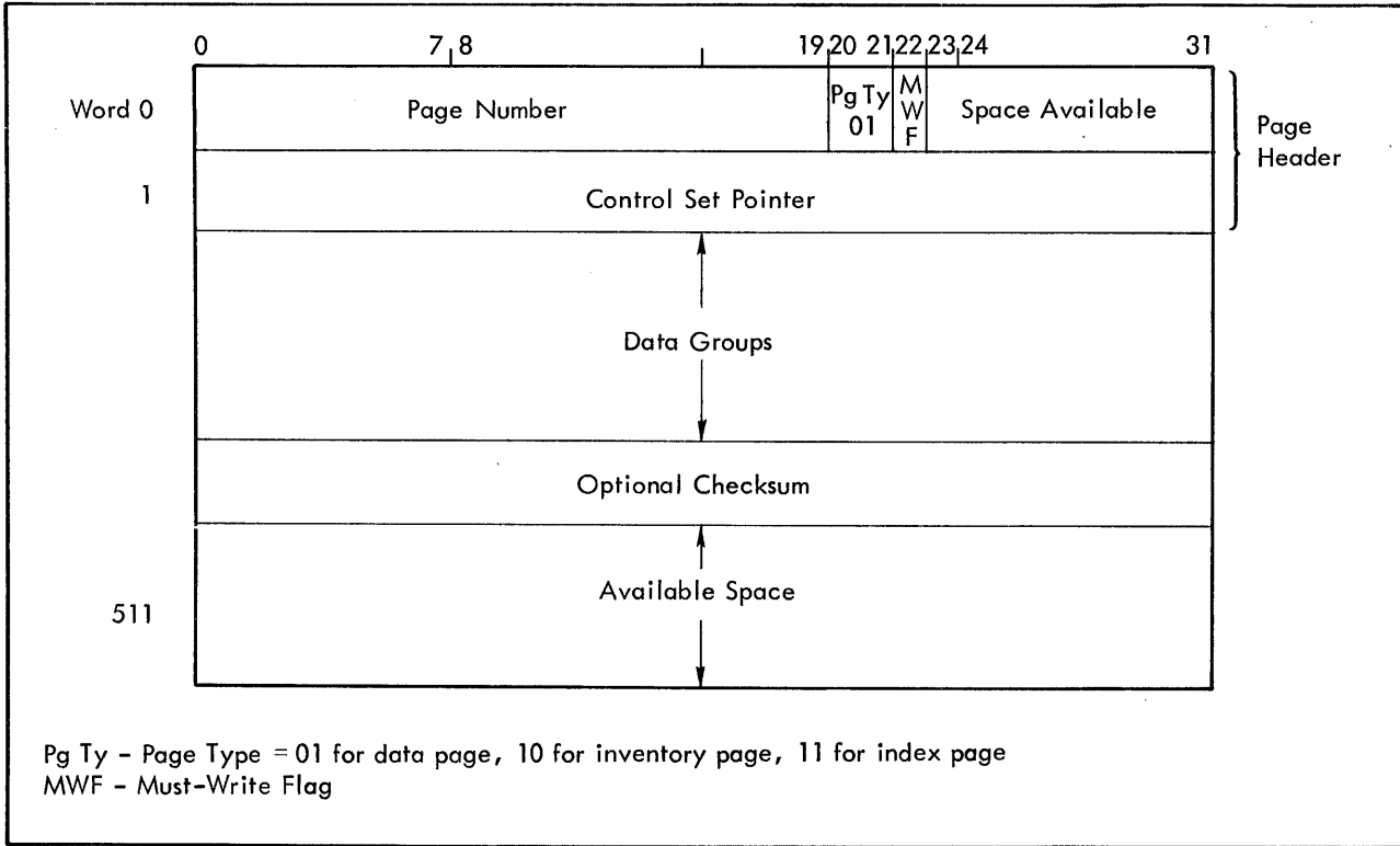
Figure D-1. Data Page Format
