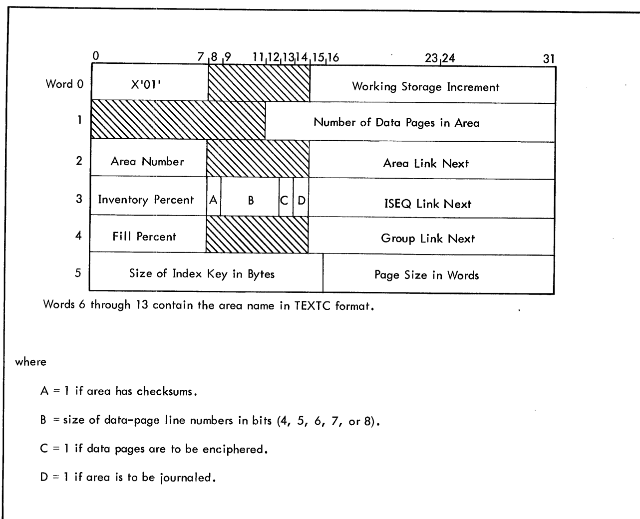
Figure B-2. Area Definition
