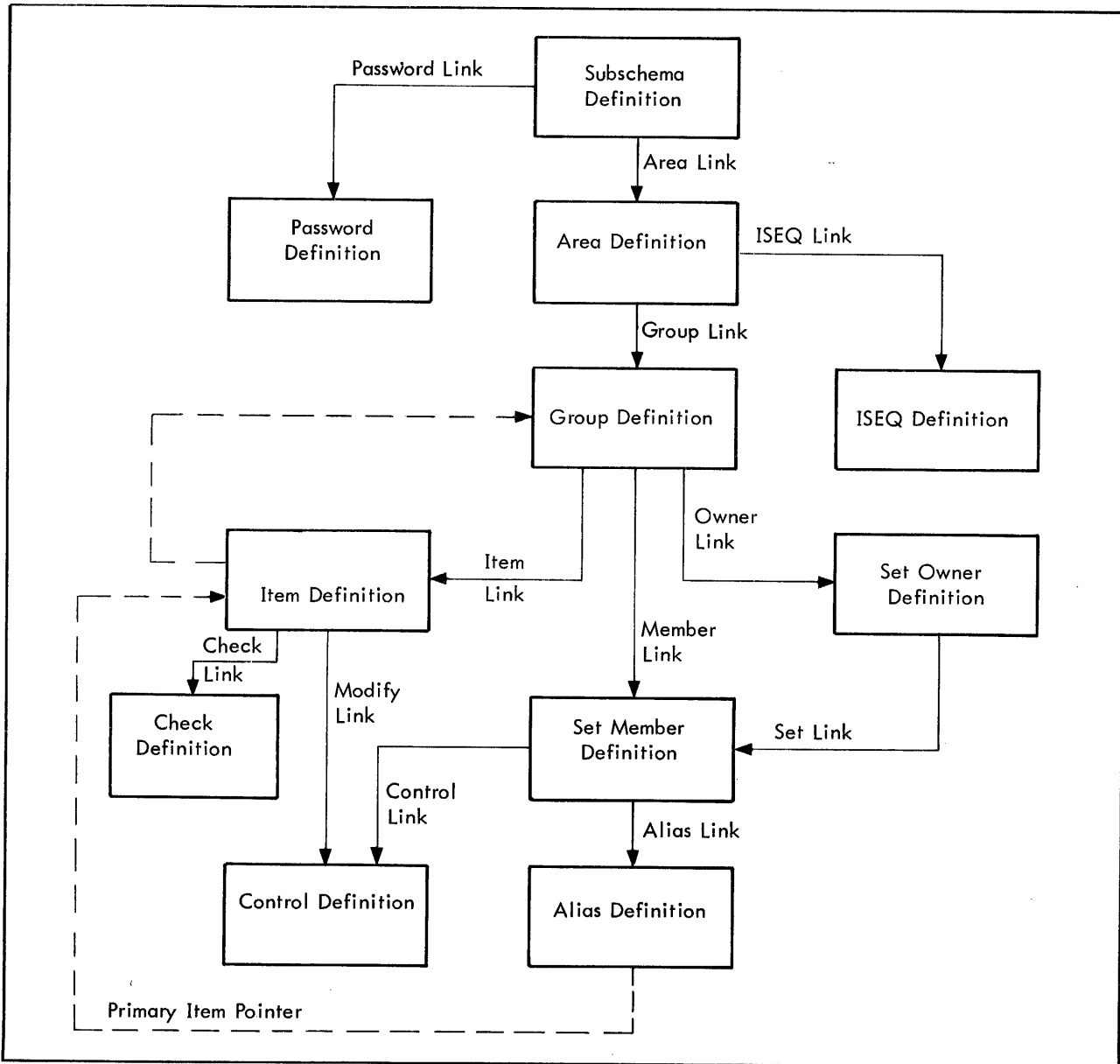
Figure B-1. Subschema Definition Structure
