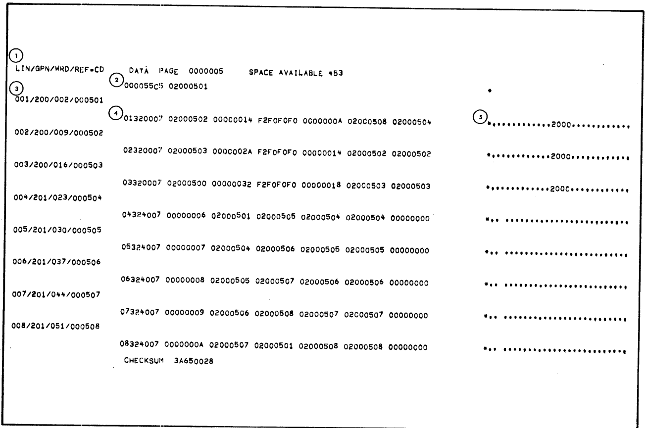
Figure 9. DMSDUMP Output Sample (Batch Job)
