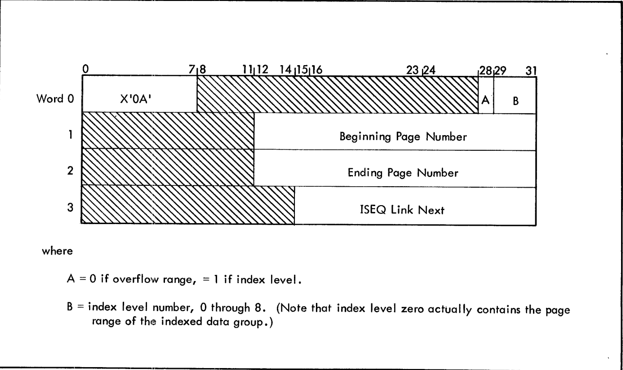
Figure B-10. Indexed-Sequential (ISEQ) Definition
