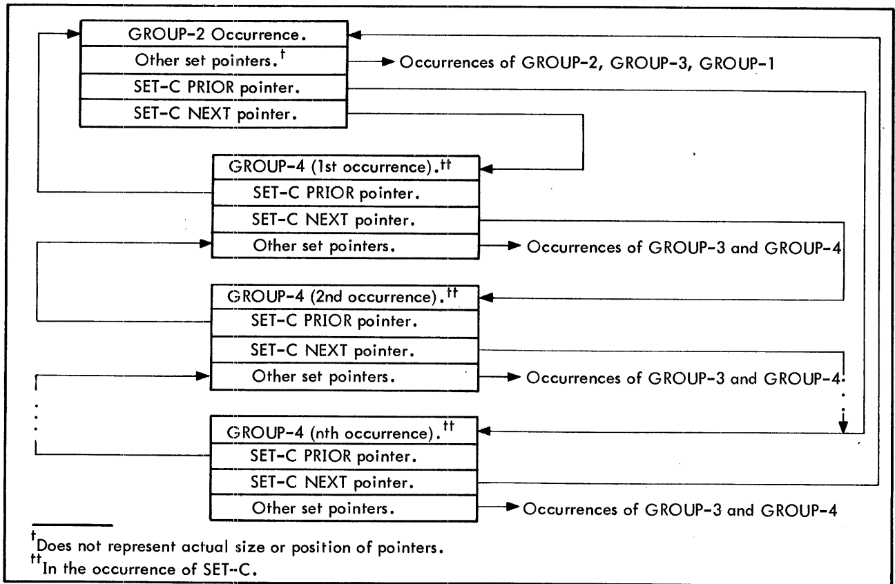
Figure 4. NEXT and PRIOR Pointers in an Occurrence of SET-C
