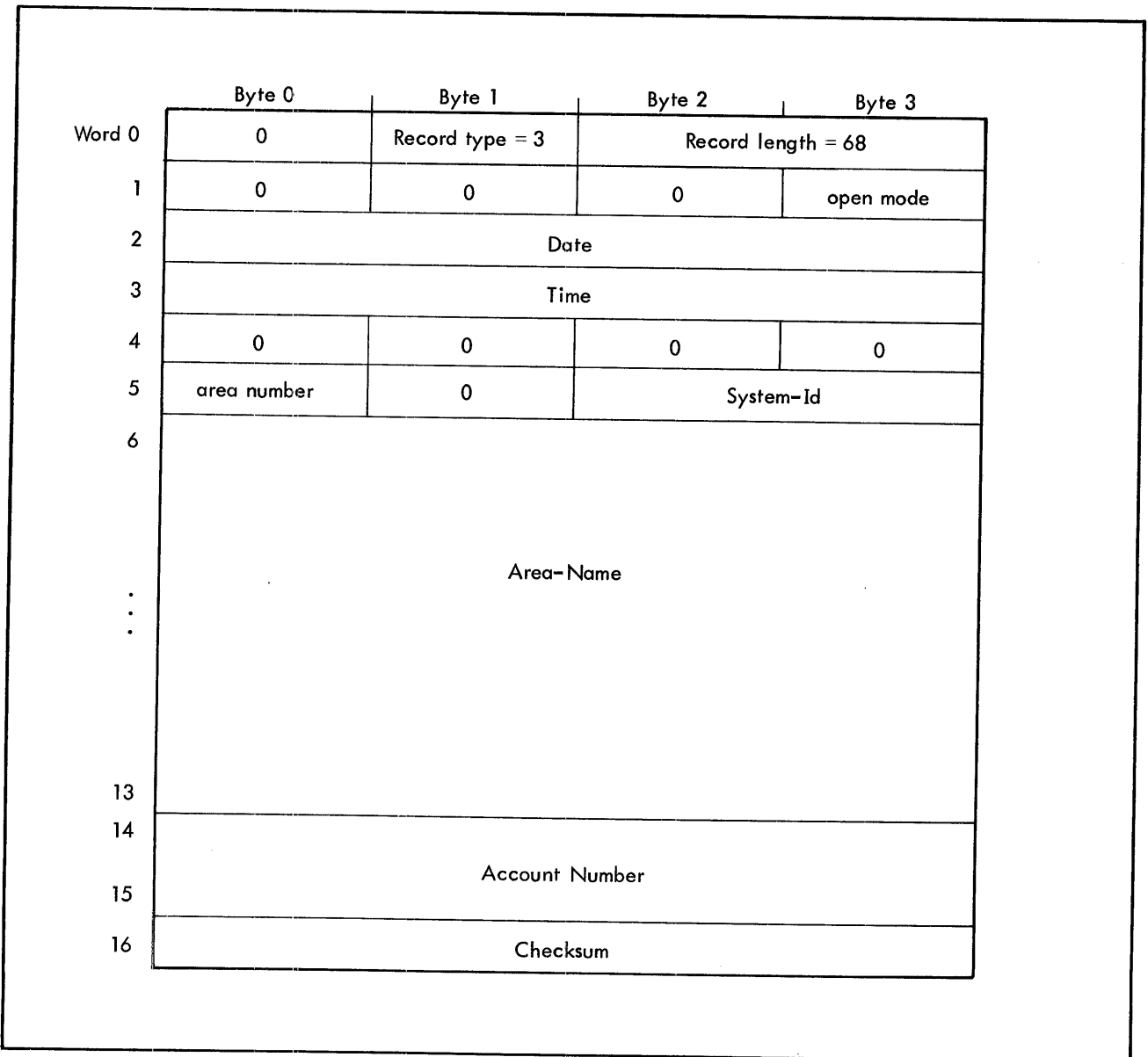
Figure E-1. Journal/Dump Begin Record
