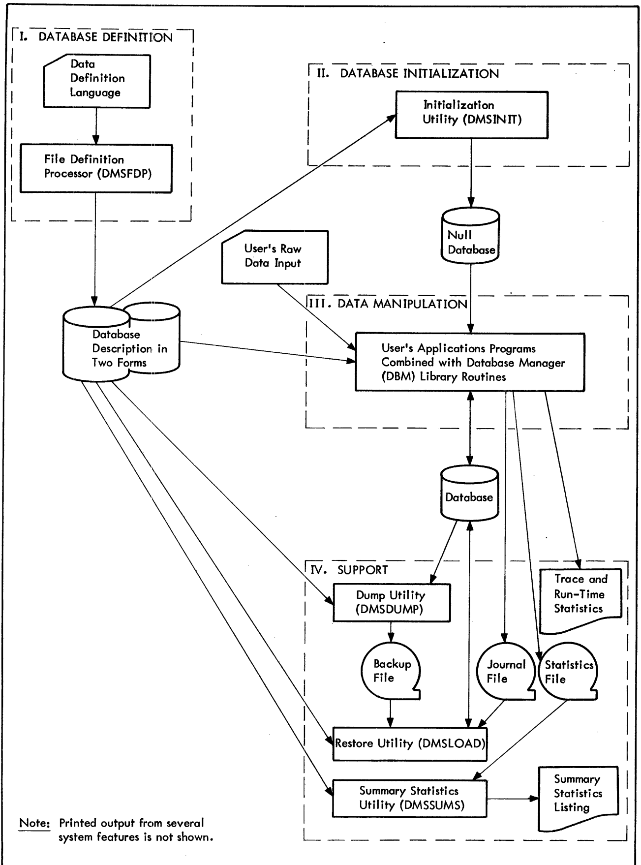
Figure 5. System Overview
