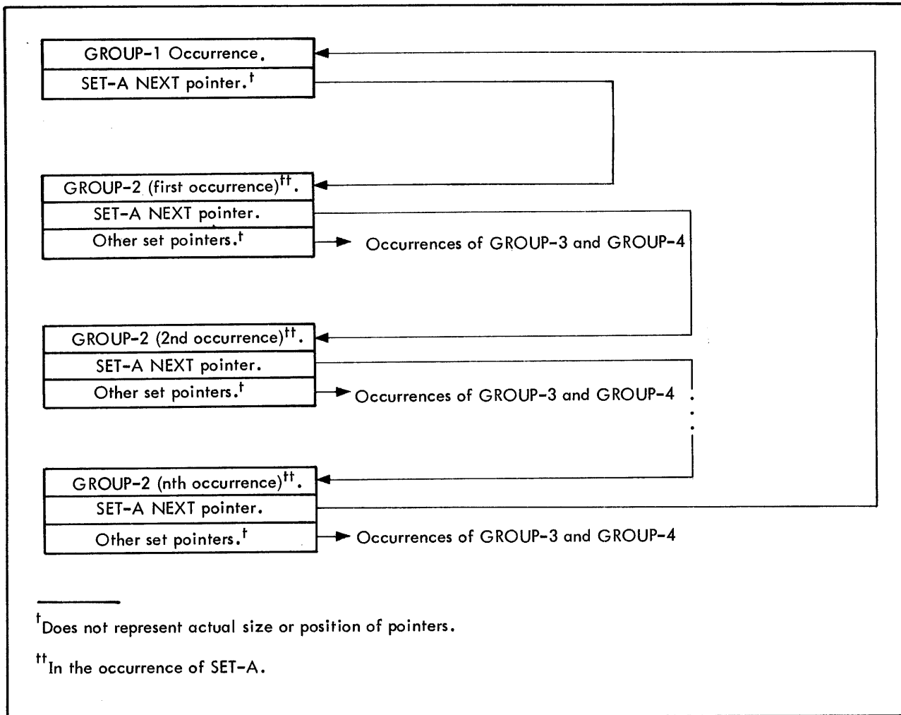
Figure 2. NEXT Pointers in an Occurrence of SET-A
