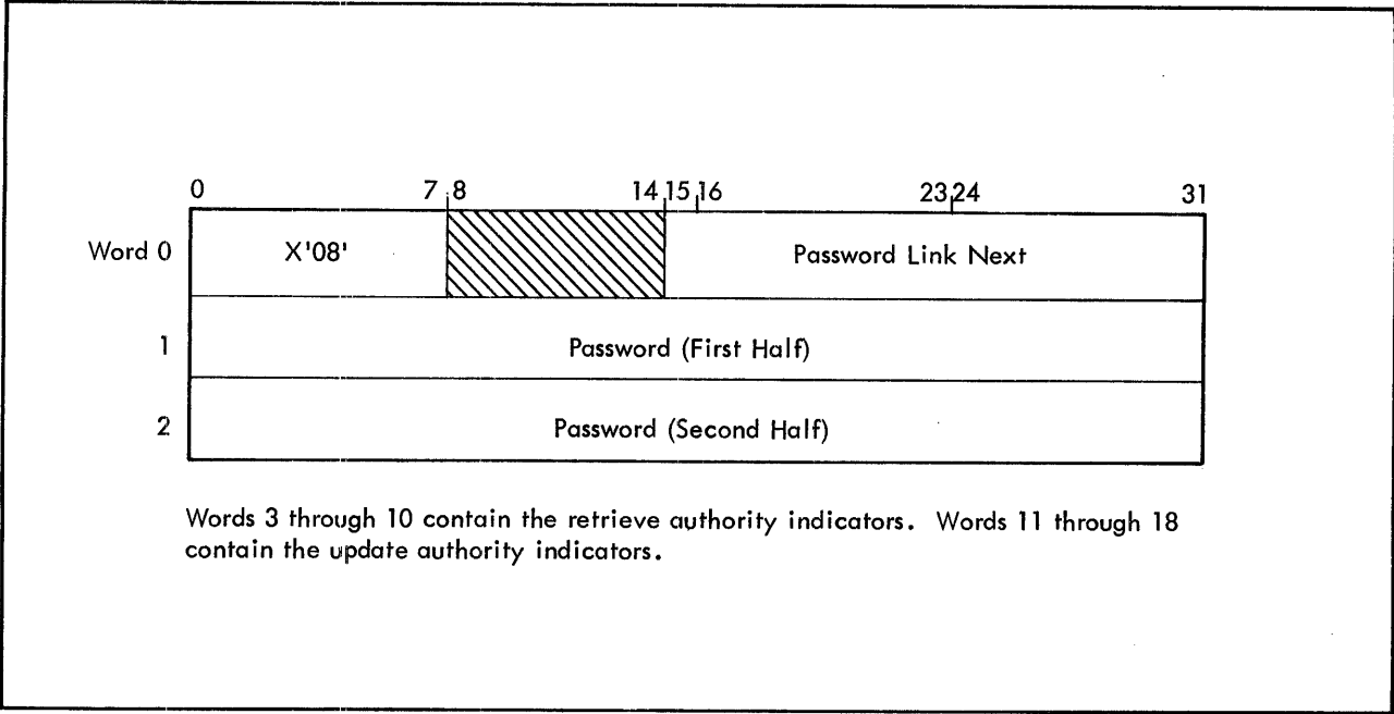
Figure B-9. Password Definition
