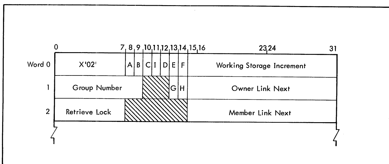
Figure B-3. Group Definition
